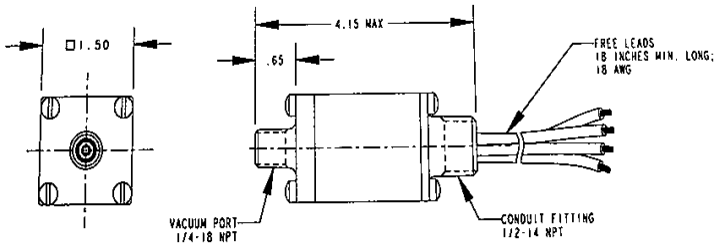
Figure 1 182P Vacuum Switch
