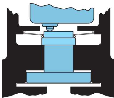
DEACTUATED
